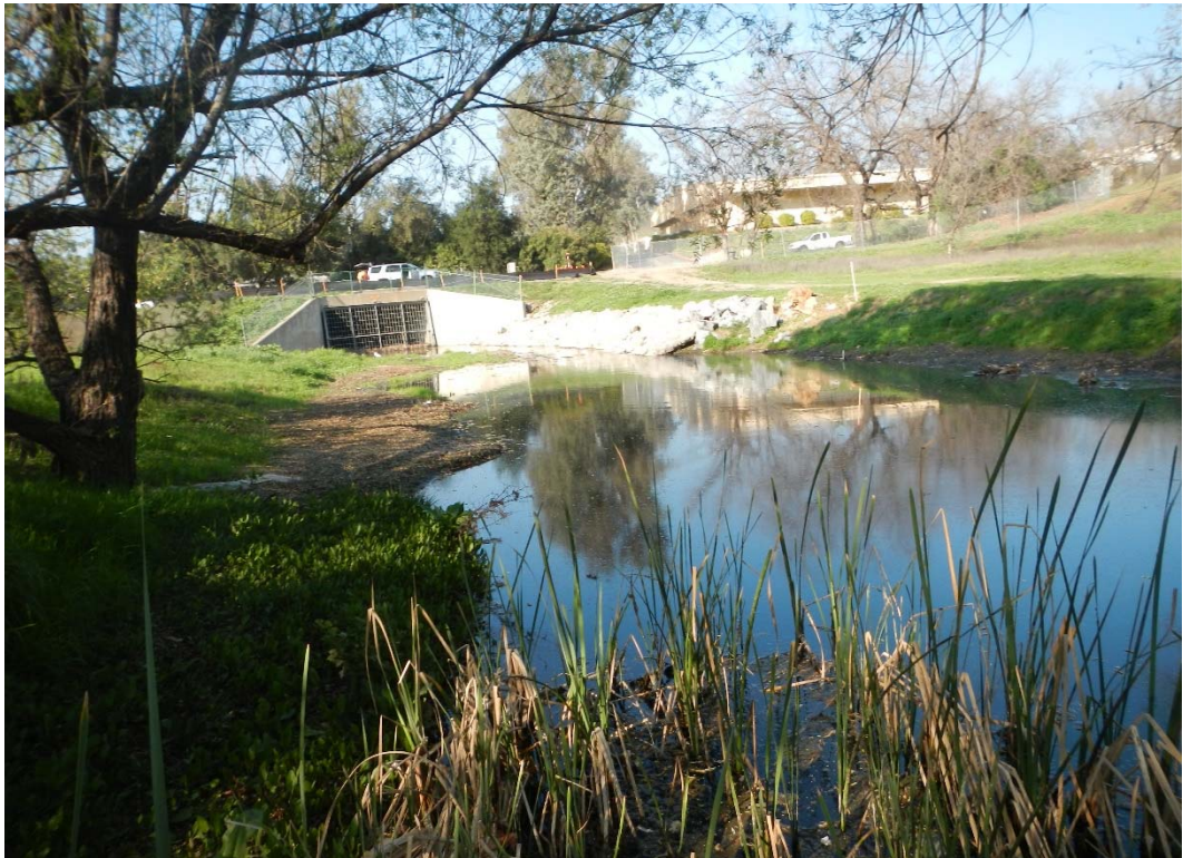
REACH DOWNSTREAM EXTENT, HEC-RAS RIVER STATION 10+35, UPSTREAM DIRECTION
